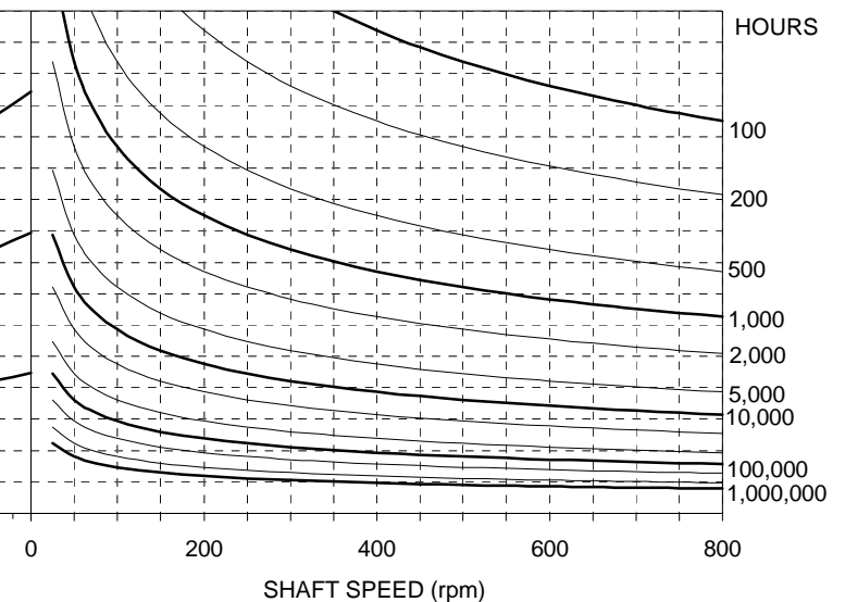
B_{10} LIFETIME
