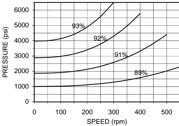
MECHANICAL EFFICIENCY
