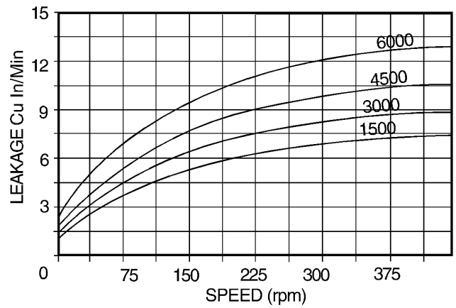
VOLUMETRIC EFFICIENCY
