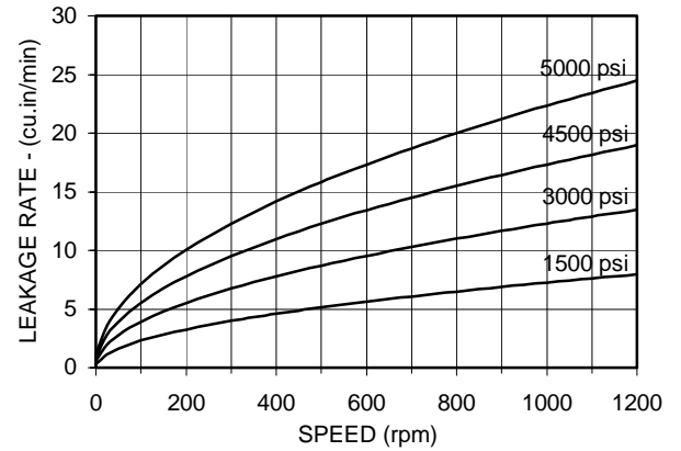
VOLUMETRIC EFFICIENCY
